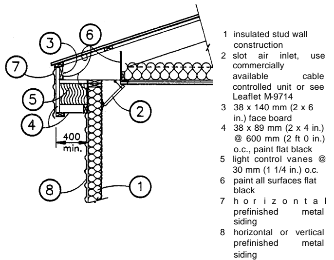
FIGURE 6 LIGHT-RESTRICTING AIR INTAKE HOOD WITH VANES (OVER-THE-PLATE)
