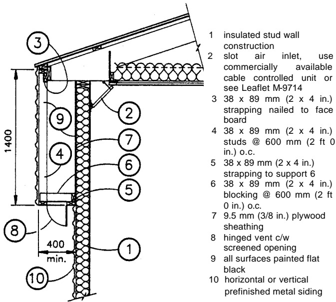
FIGURE 4 LIGHT-RESTRICTING AIR INTAKE HOOD AT EAVE
