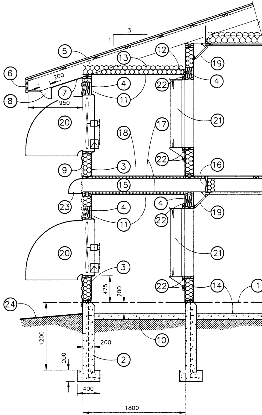
FIGURE 3. LIGHT-RESTRICTING FAN HOUSE FOR A TWO-STORY BARN
