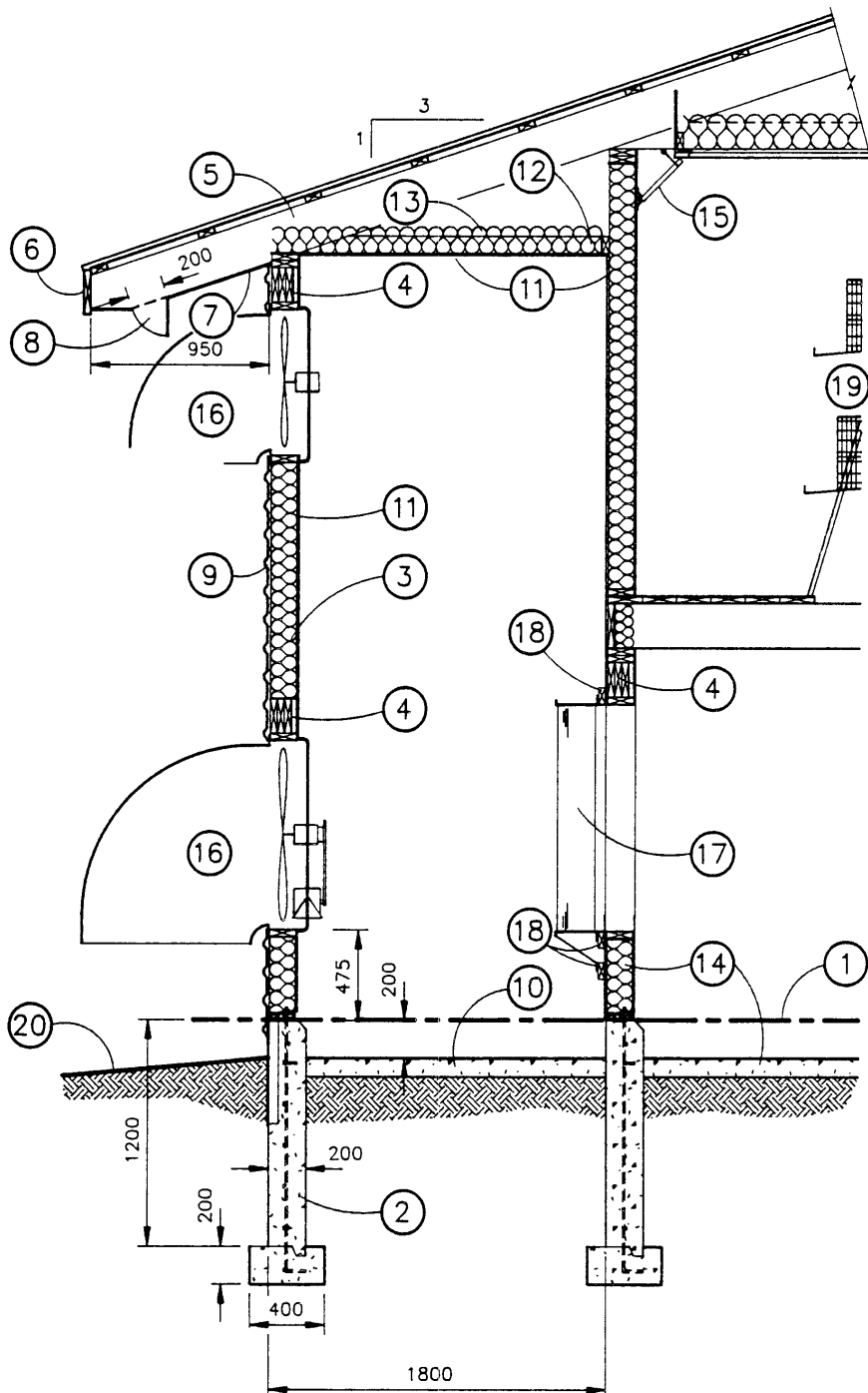
FIGURE 2. LIGHT-RESTRICTING FAN HOUSE FOR A HIGH RISE LAYER BARN
