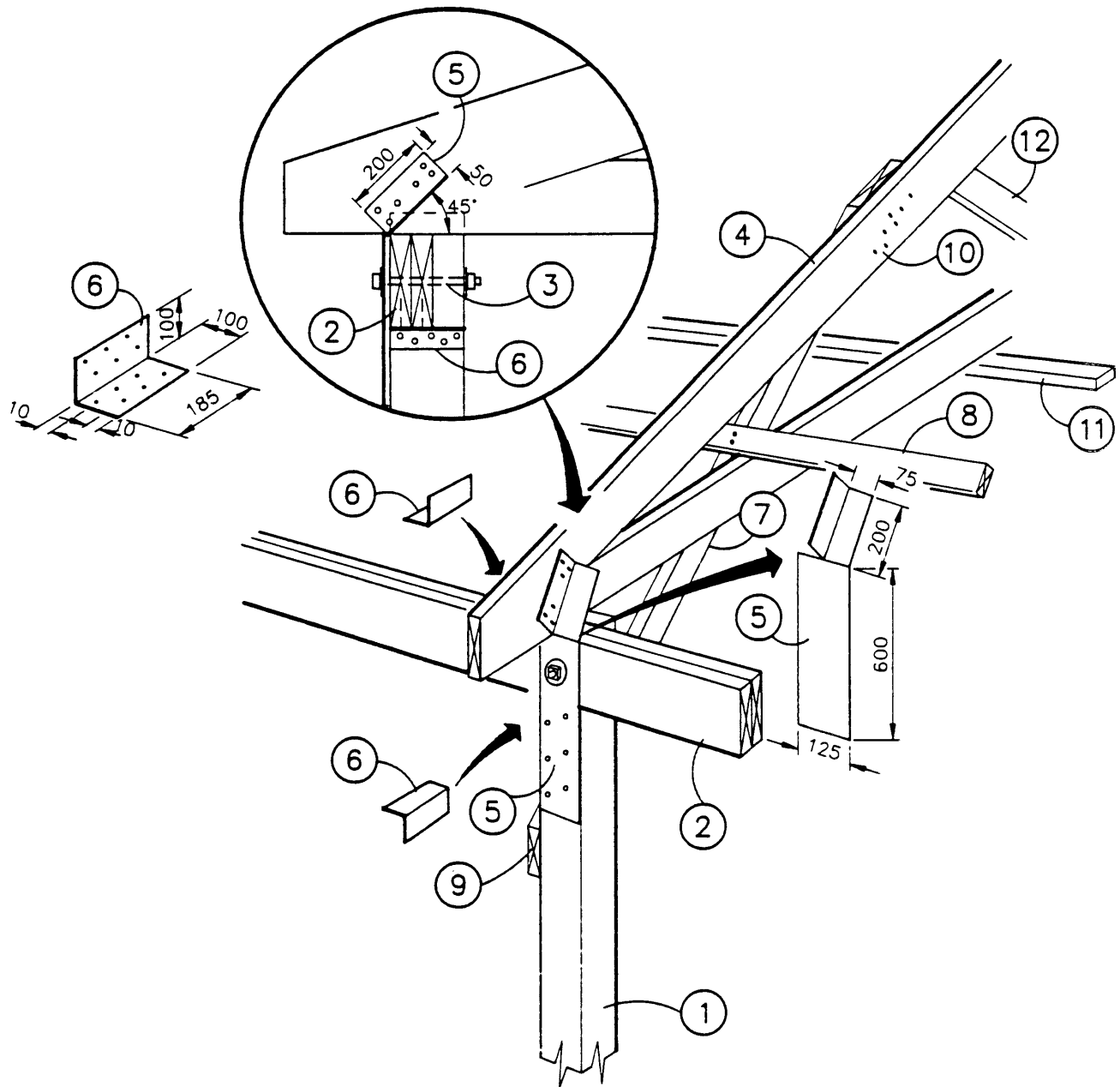
FIGURE 3 POLE FRAMES WITH PLATE MEMBERS NOTCHED INTO POLE
