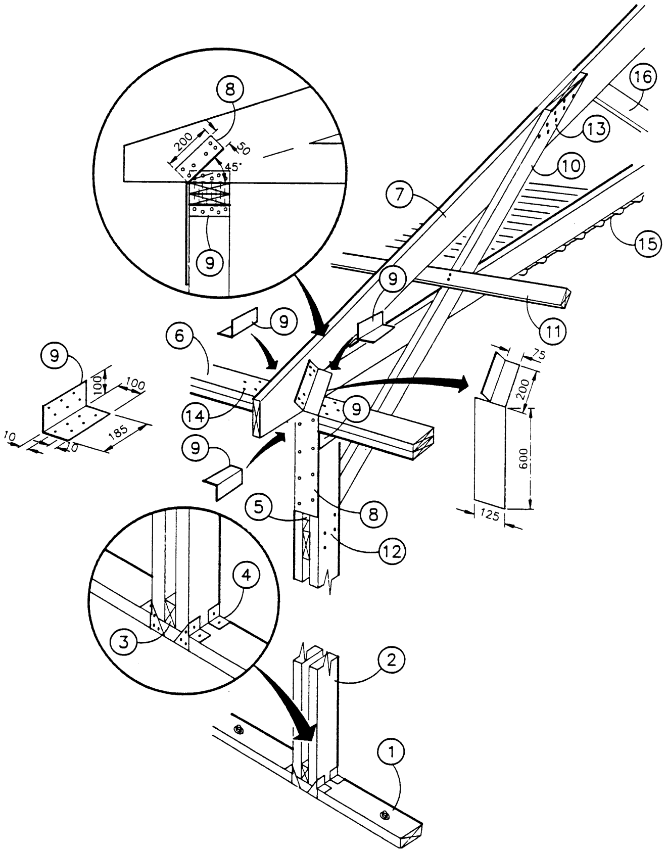
FIGURE 2 HEAVY DUTY KNEE-BRACES FOR STUD WALLS
