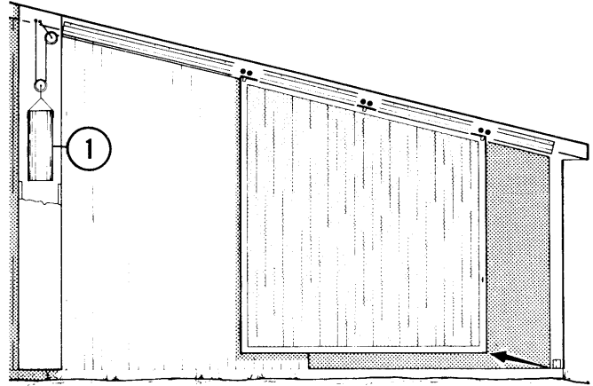
Figure 7 Door on inclined track. The counterweight 1 travels half the distance travelled by the door
