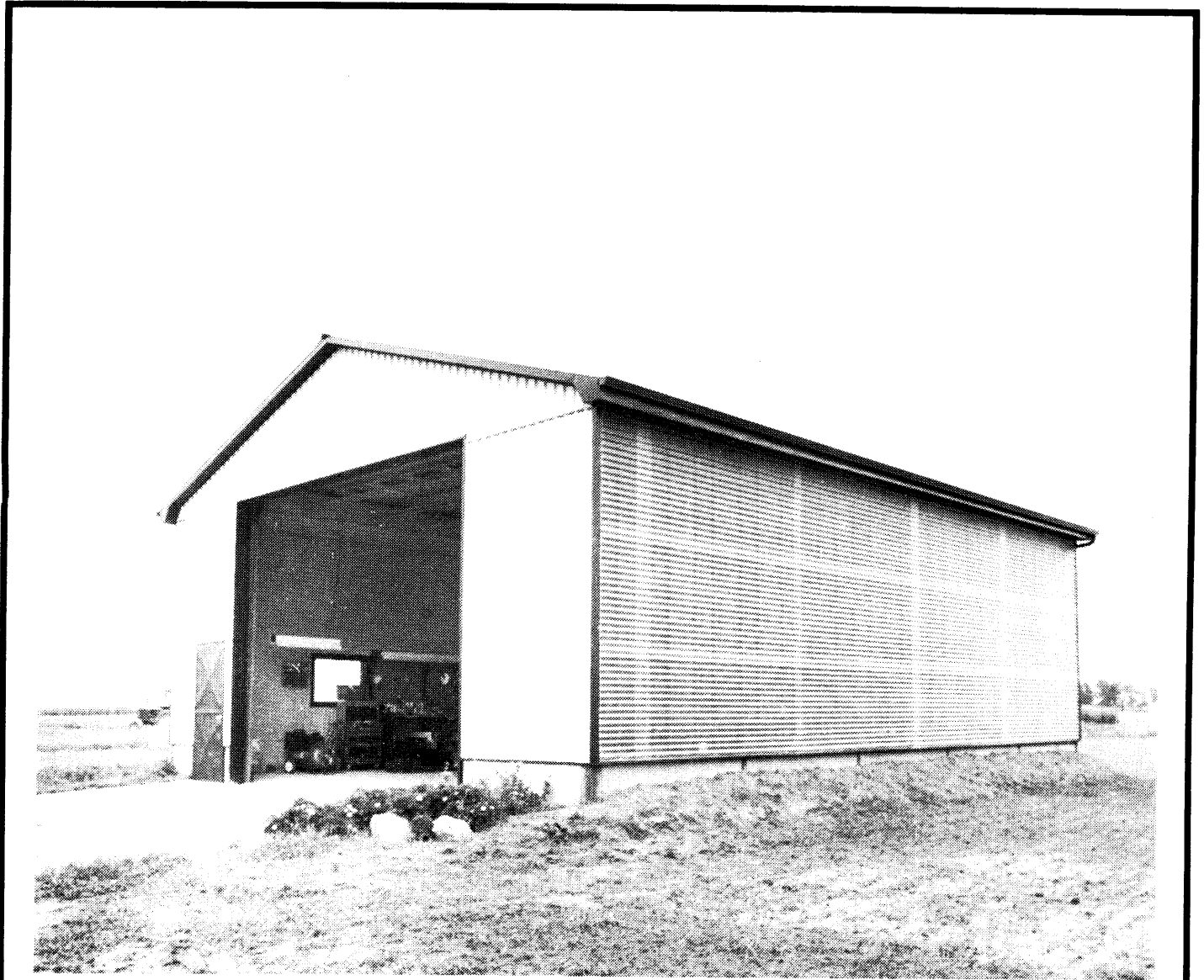
Figure 1. Farm workshop showing a passive solar collector on the south facing wall. Natural air movement circulates the absorbed heat into the shop area.
